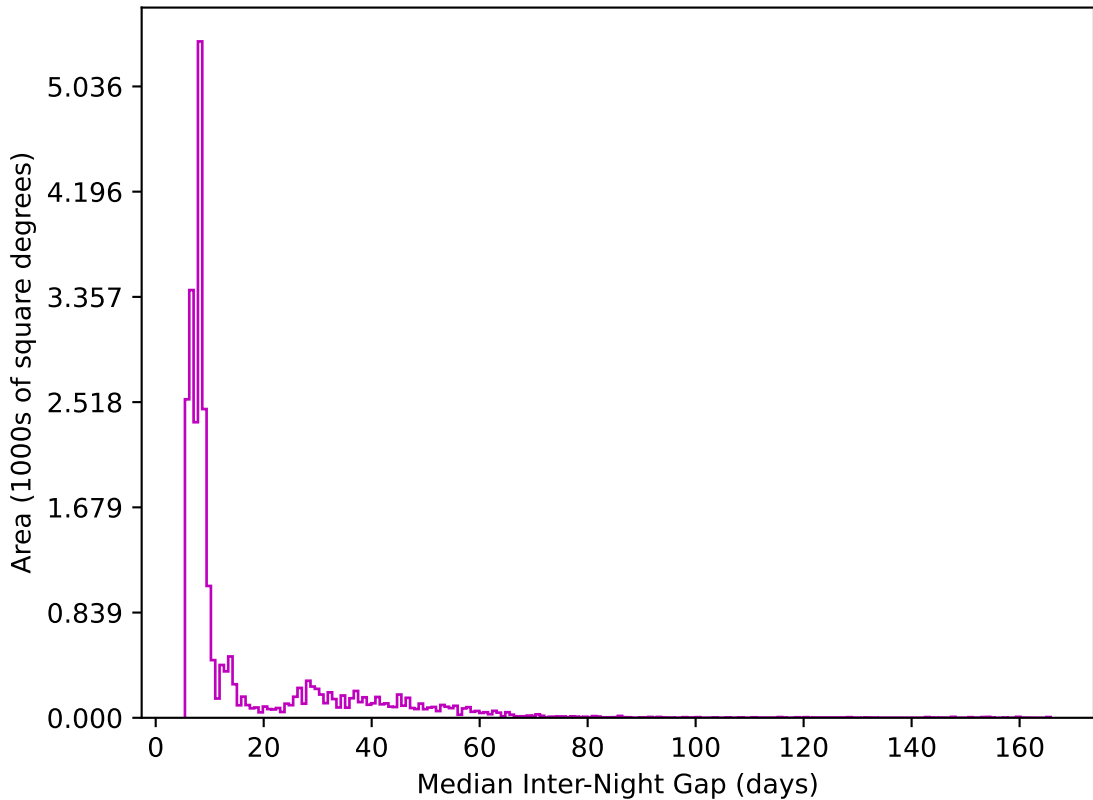
weather_cloudso0v3.4_10yrs All sky z band: Median Inter-Night Gap
