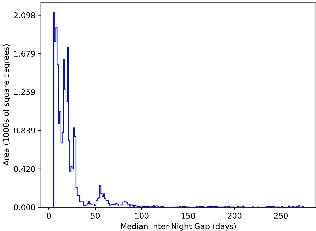
weather_cloudso0v3.4_10yrs All sky y band: Median Inter-Night Gap
