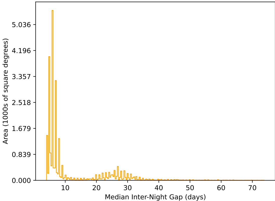
weather_cloudso0v3.4_10yrs All sky r band: Median Inter-Night Gap
