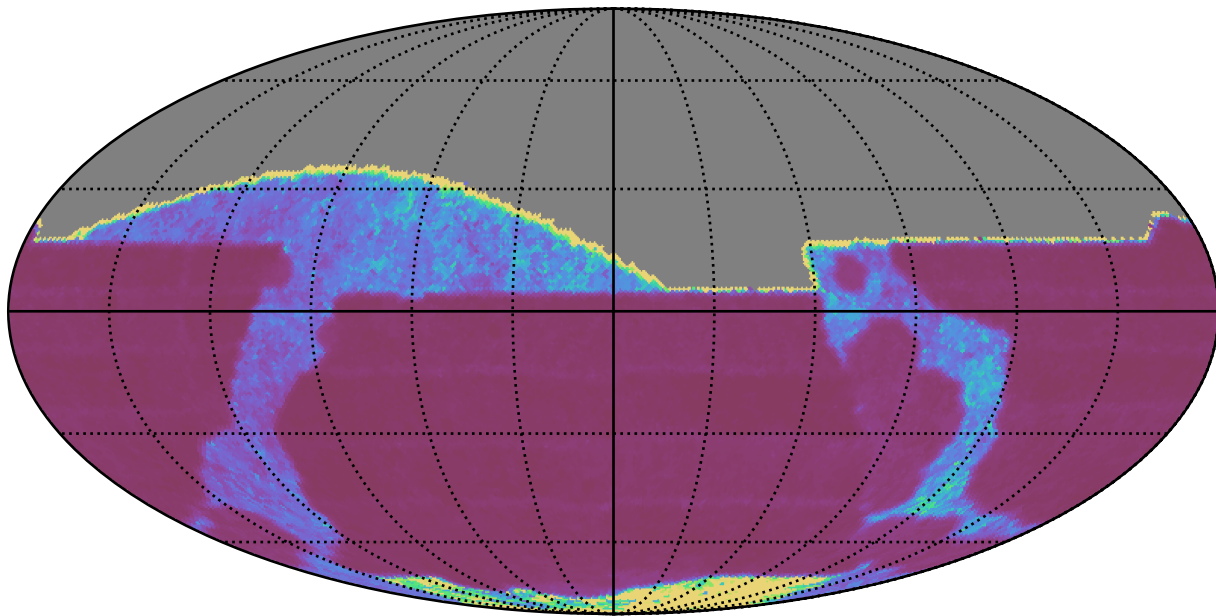
weather_cloudso0v3.4_10yrs All sky i band: Median Inter-Night Gap
