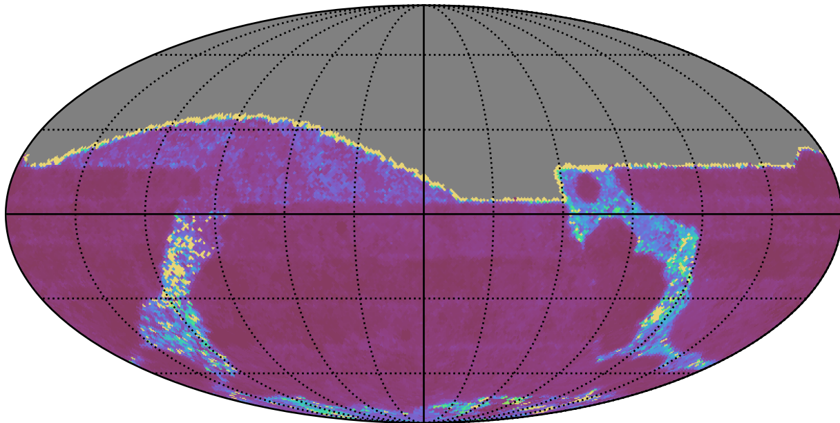
weather_cloudso0v3.4_10yrs All sky g band: Median Inter-Night Gap
