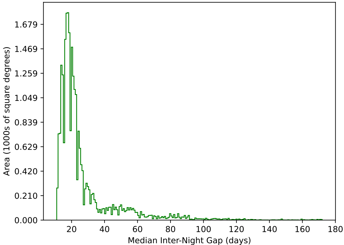
weather_cloudso0v3.4_10yrs All sky g band: Median Inter-Night Gap
