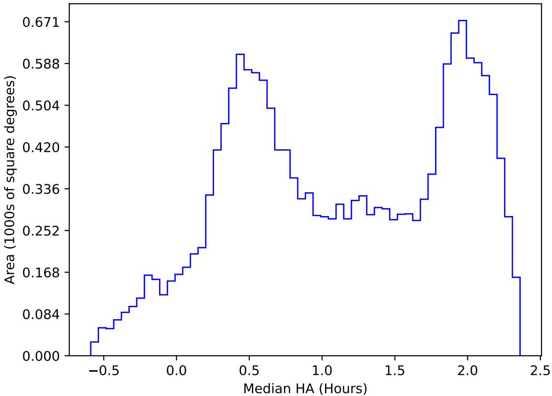
weather_cloudso0v3.4_10yrs WFD z band: Median HA
