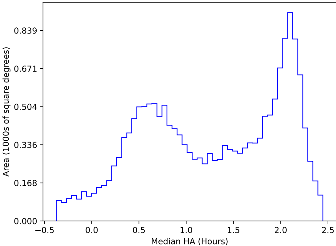
weather_cloudso0v3.4_10yrs WFD y band: Median HA
