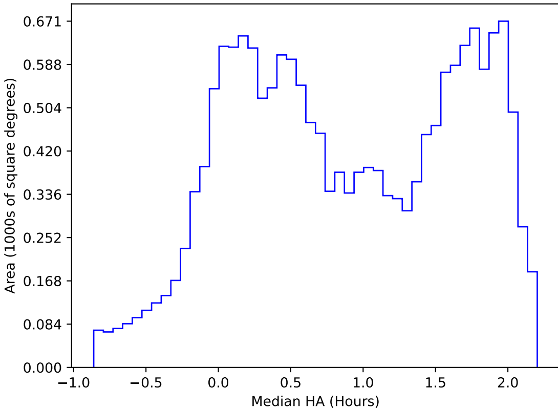
weather_cloudso0v3.4_10yrs WFD r band: Median HA
