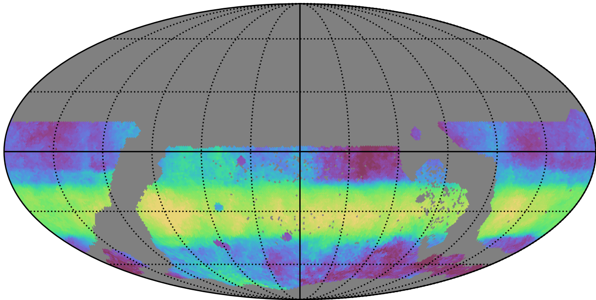
weather_cloudso0v3.4_10yrs WFD i band: Median HA
