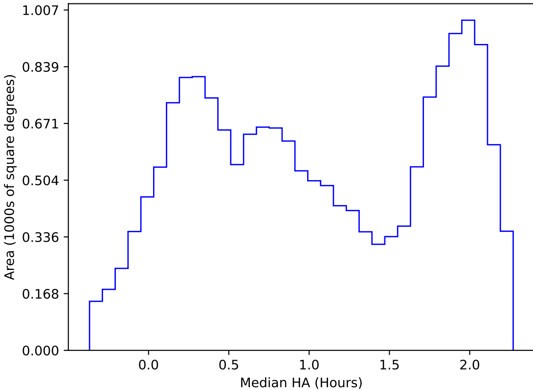
weather_cloudso0v3.4_10yrs WFD i band: Median HA
