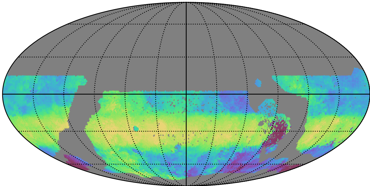
weather_cloudso0v3.4_10yrs WFD g band: Median HA
