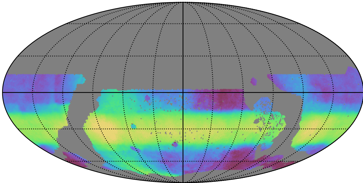
weather_cloudso0v3.4_10yrs WFD all bands: Median HA
