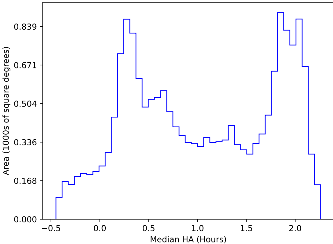
weather_cloudso0v3.4_10yrs WFD all bands: Median HA
