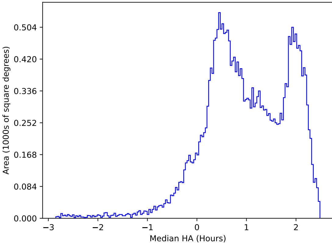
weather_cloudso0v3.4_10yrs All sky z band: Median HA
