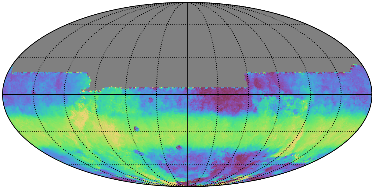
weather_cloudso0v3.4_10yrs All sky y band: Median HA
