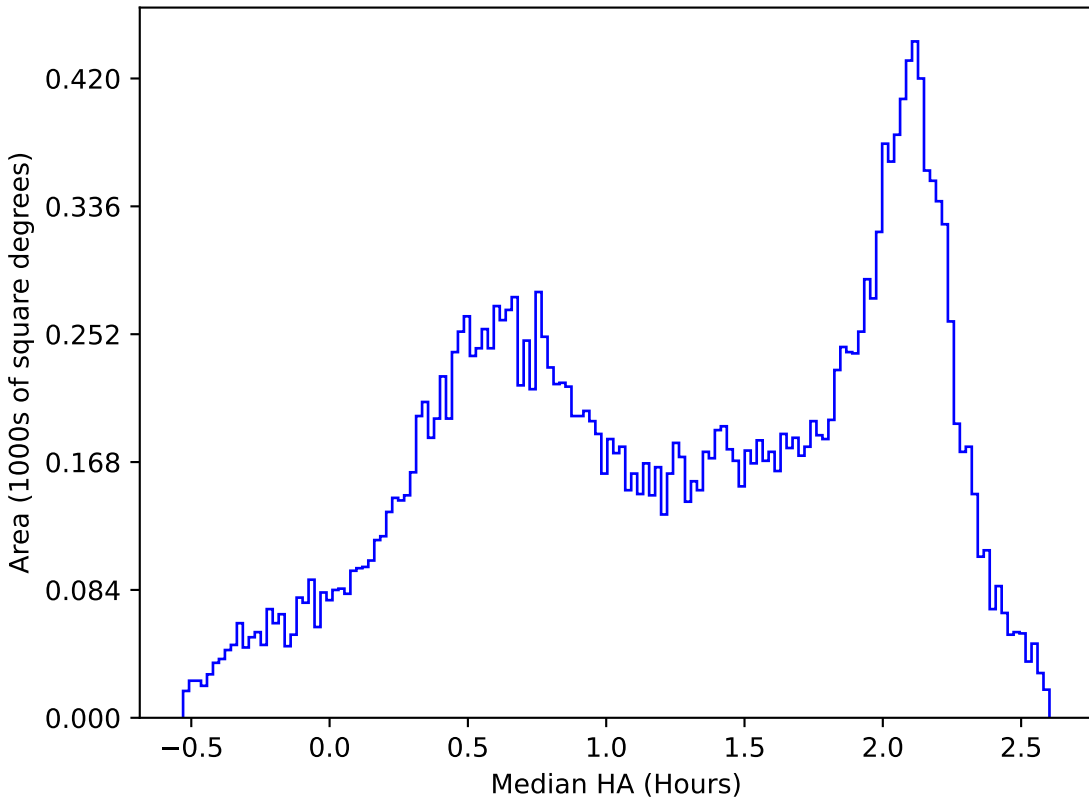
weather_cloudso0v3.4_10yrs All sky y band: Median HA
