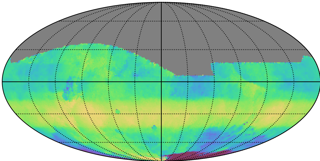
weather_cloudso0v3.4_10yrs All sky r band: Median HA
