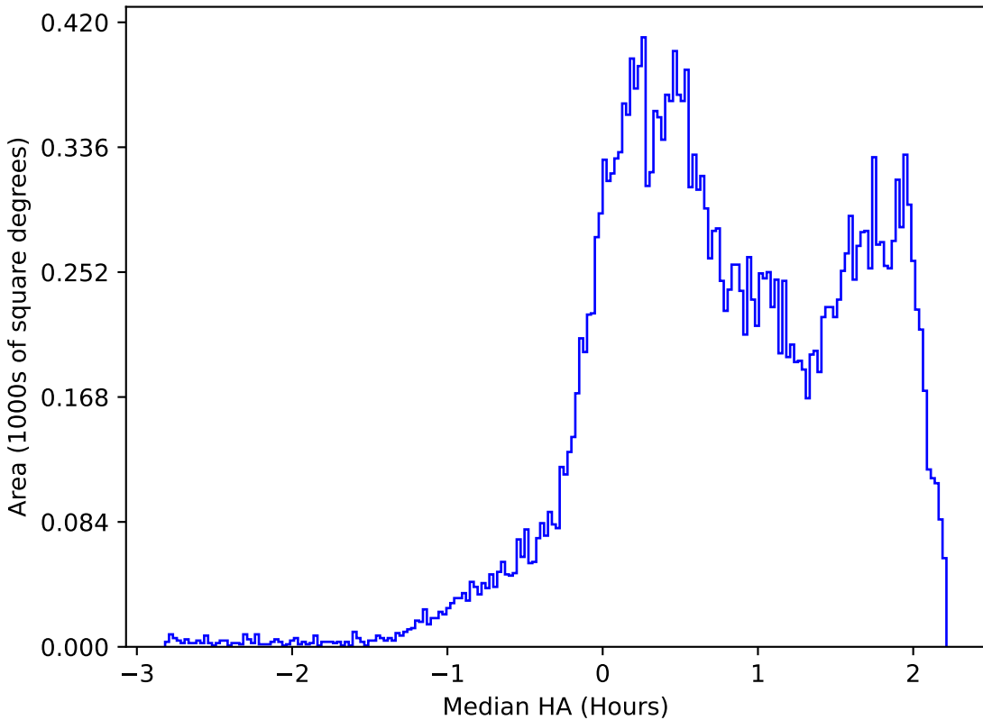
weather_cloudso0v3.4_10yrs All sky r band: Median HA
