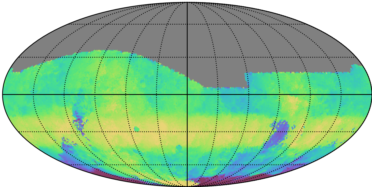
weather_cloudso0v3.4_10yrs All sky g band: Median HA
