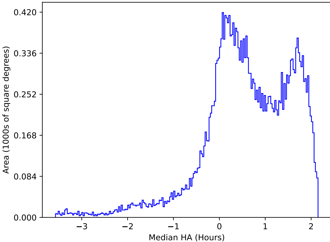
weather_cloudso0v3.4_10yrs All sky g band: Median HA
