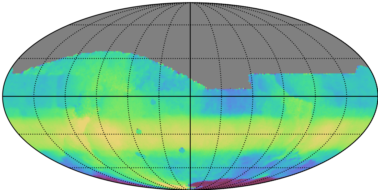
weather_cloudso0v3.4_10yrs All sky all bands: Median HA
