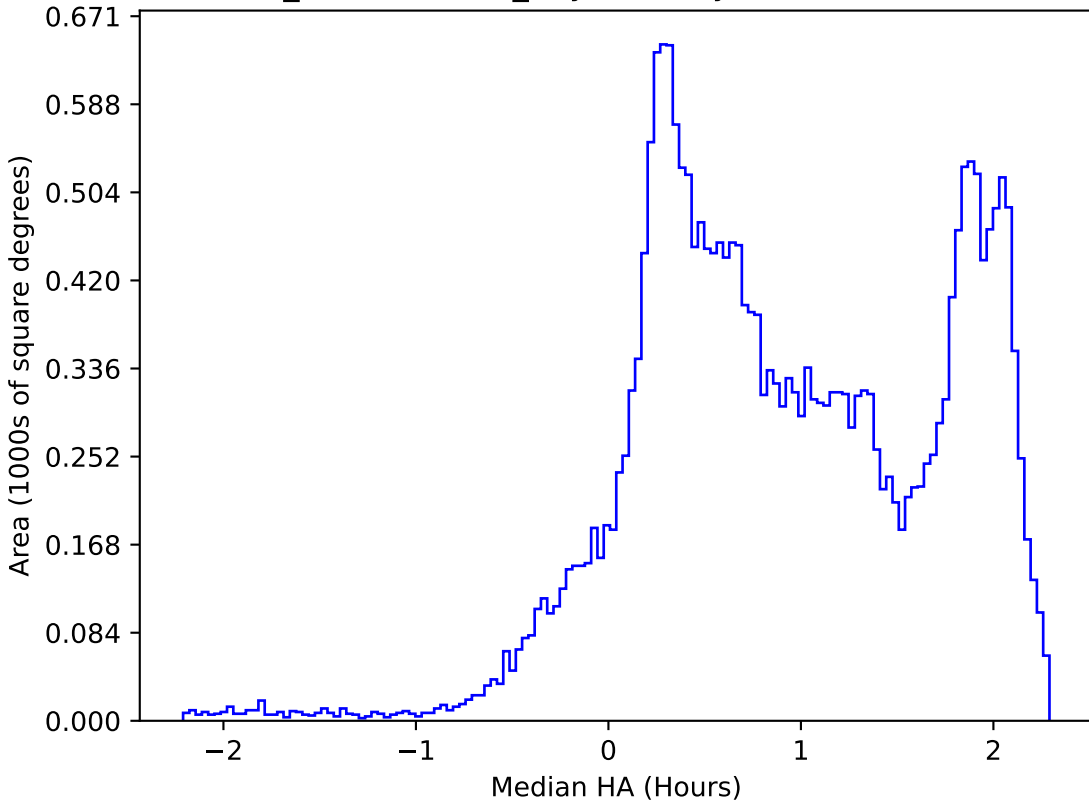
weather_cloudso0v3.4_10yrs All sky all bands: Median HA
