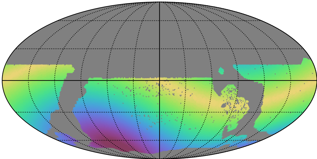
weather_cloudso0v3.4_10yrs WFD r band: Max solarElong
