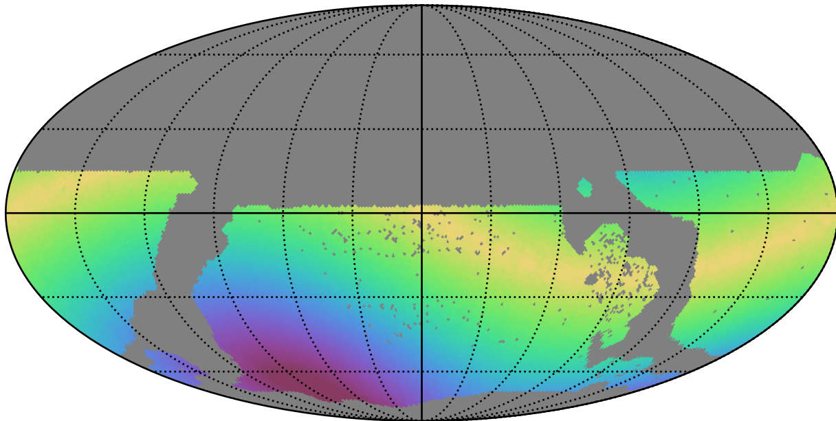
weather_cloudso0v3.4_10yrs WFD g band: Max solarElong
