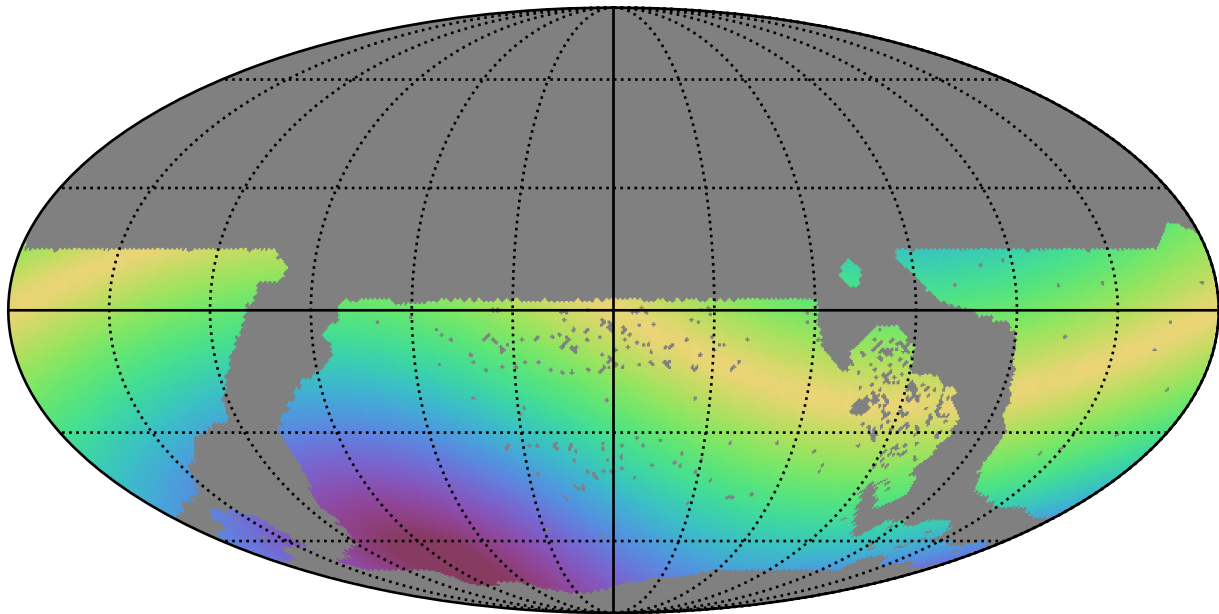
weather_cloudso0v3.4_10yrs WFD all bands: Max solarElong
