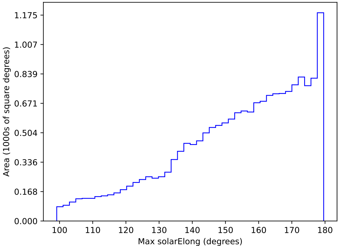
weather_cloudso0v3.4_10yrs WFD all bands: Max solarElong
