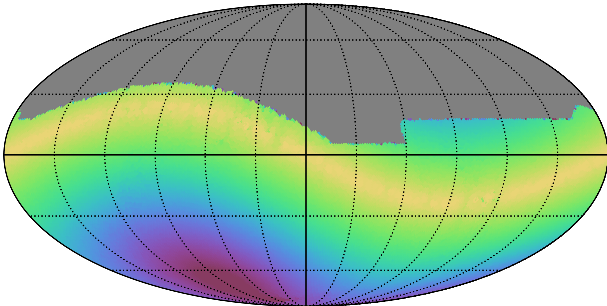
weather_cloudso0v3.4_10yrs All sky z band: Max solarElong
