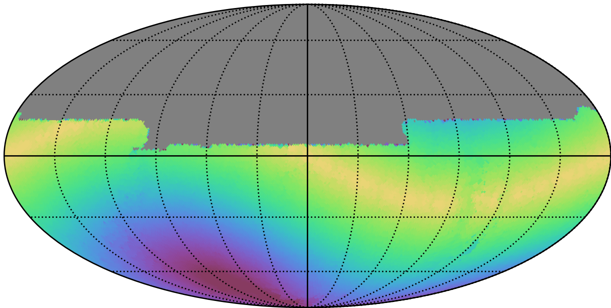
weather_cloudso0v3.4_10yrs All sky u band: Max solarElong
