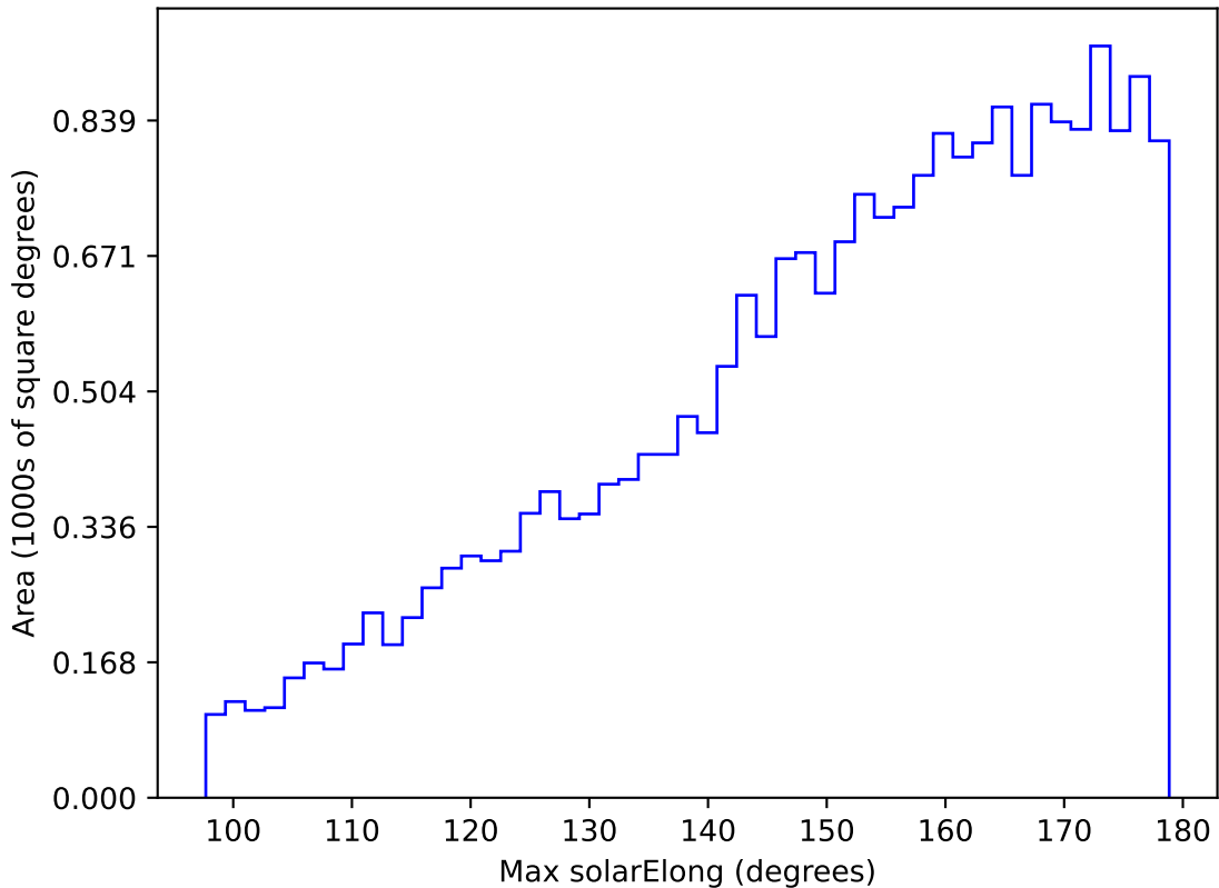
weather_cloudso0v3.4_10yrs All sky u band: Max solarElong
