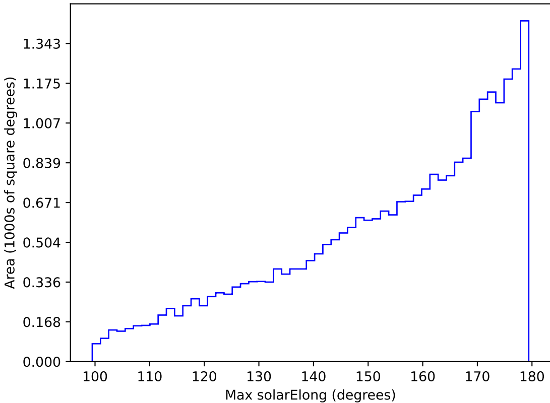
weather_cloudso0v3.4_10yrs All sky r band: Max solarElong
