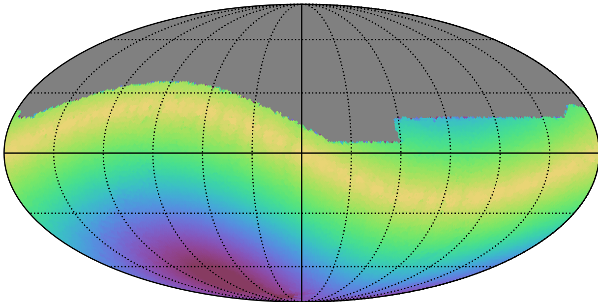
weather_cloudso0v3.4_10yrs All sky g band: Max solarElong
