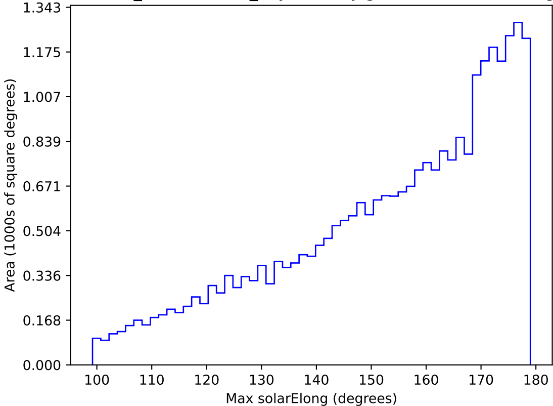
weather_cloudso0v3.4_10yrs All sky g band: Max solarElong
