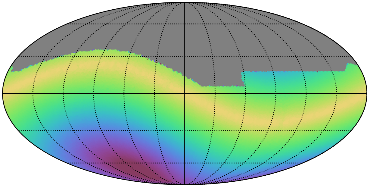
weather_cloudso0v3.4_10yrs All sky all bands: Max solarElong
