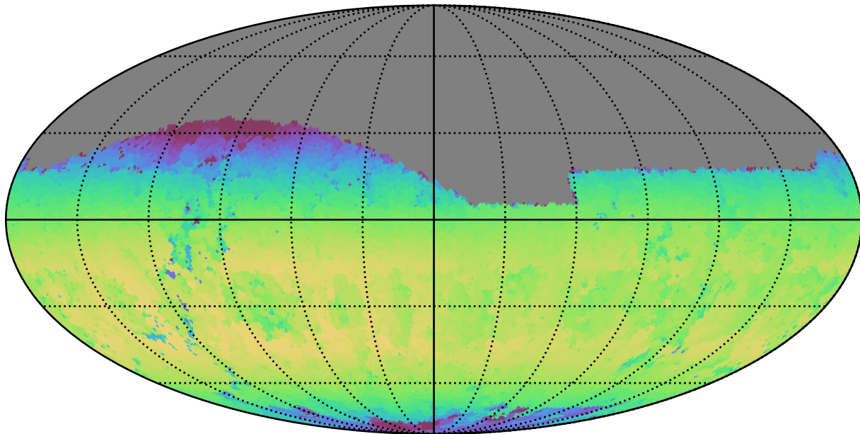
weather_cloudso0v3.4_10yrs Yr 1 z band: Max skyBrightness
