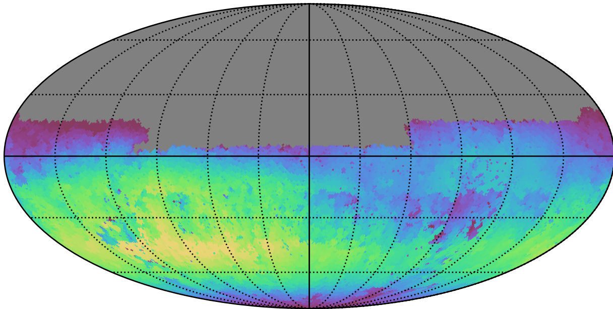
weather_cloudso0v3.4_10yrs Yr 1 u band: Max skyBrightness
