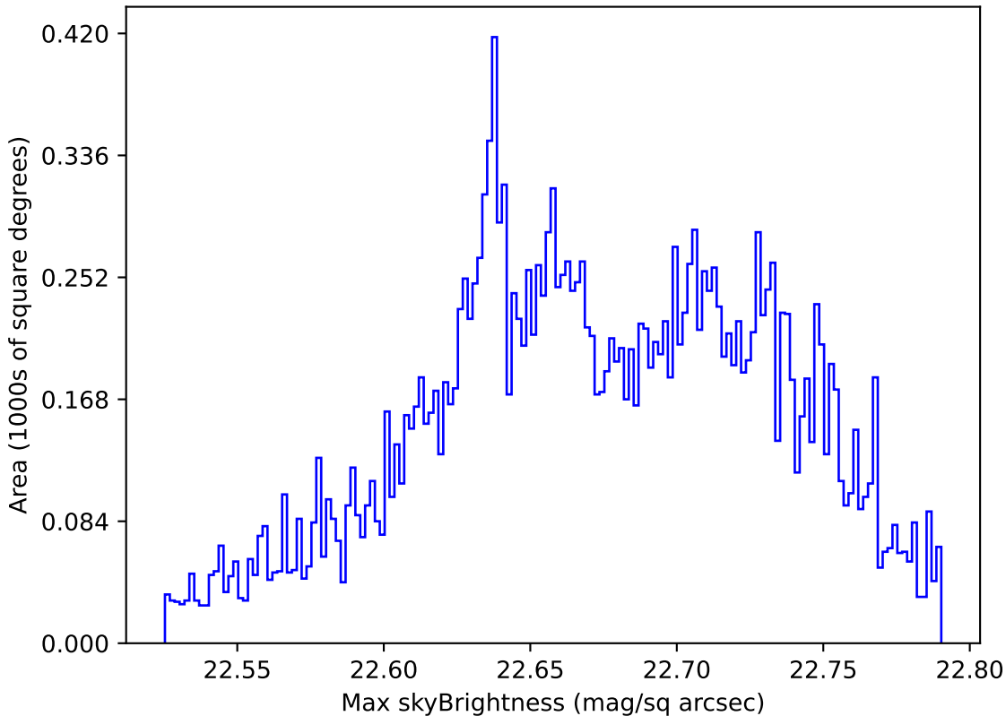
weather_cloudso0v3.4_10yrs Yr 1 u band: Max skyBrightness
