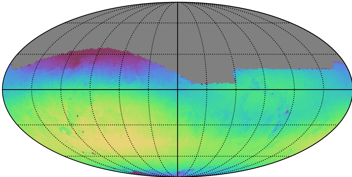
weather_cloudso0v3.4_10yrs Yr 1 r band: Max skyBrightness
