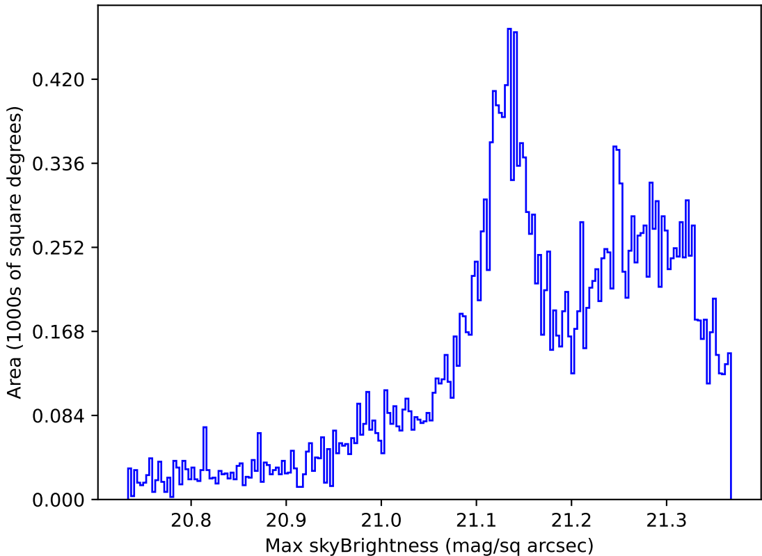
weather_cloudso0v3.4_10yrs Yr 1 r band: Max skyBrightness
