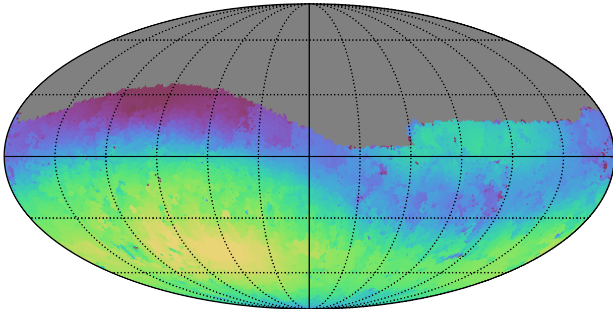
weather_cloudso0v3.4_10yrs Yr 1 g band: Max skyBrightness
