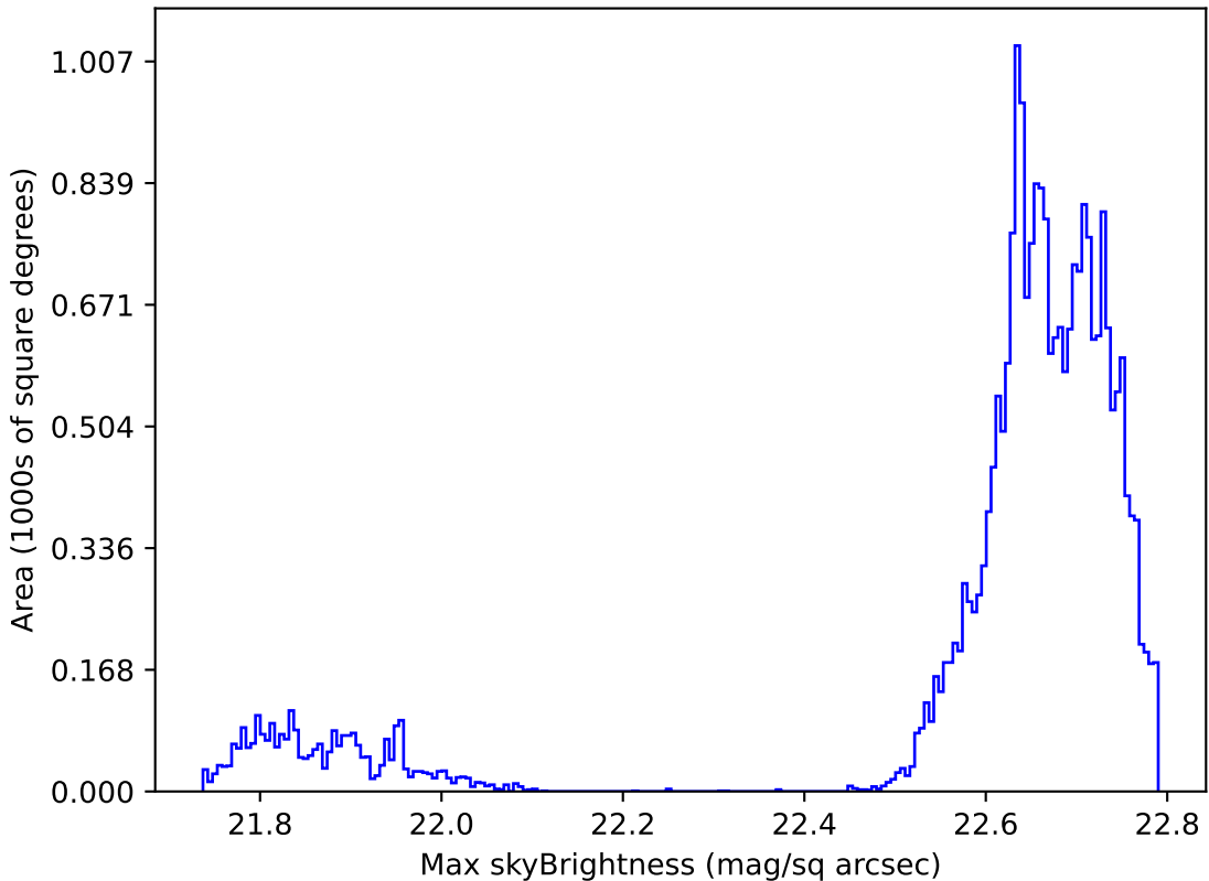
weather_cloudso0v3.4_10yrs Yr 1 all bands: Max skyBrightness
