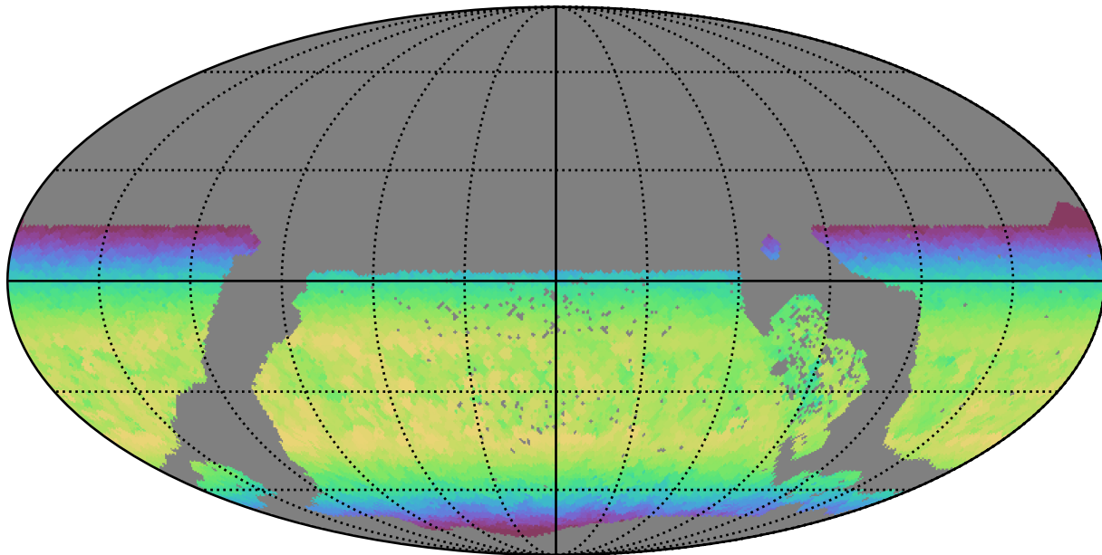
weather_cloudso0v3.4_10yrs WFD y band: Max skyBrightness
