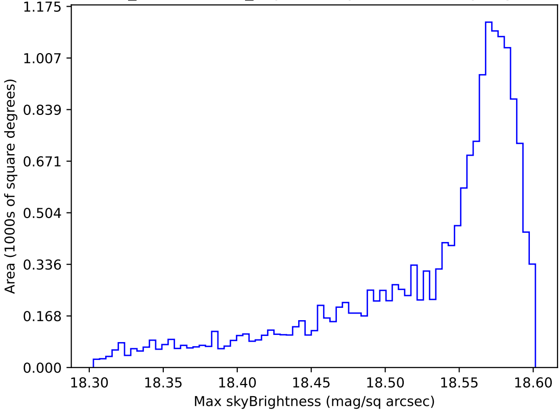
weather_cloudso0v3.4_10yrs WFD y band: Max skyBrightness
