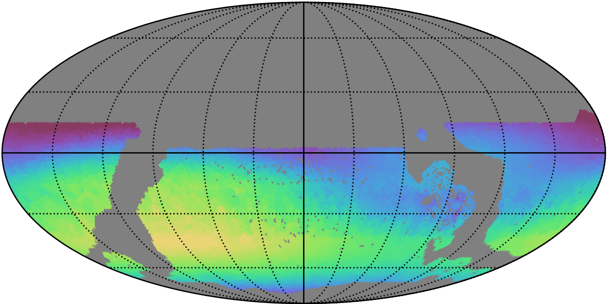
weather_cloudso0v3.4_10yrs WFD u band: Max skyBrightness
