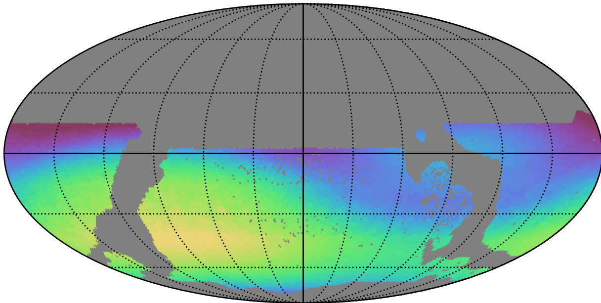
weather_cloudso0v3.4_10yrs WFD r band: Max skyBrightness
