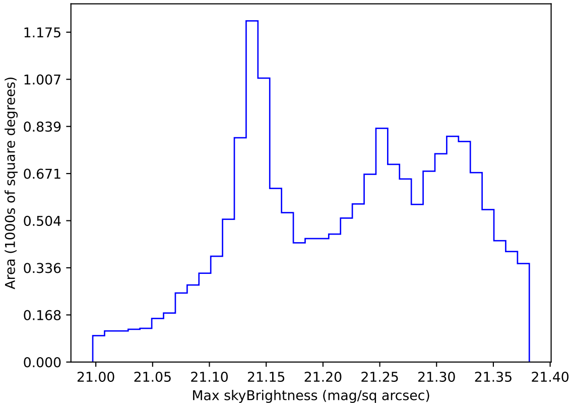
weather_cloudso0v3.4_10yrs WFD r band: Max skyBrightness
