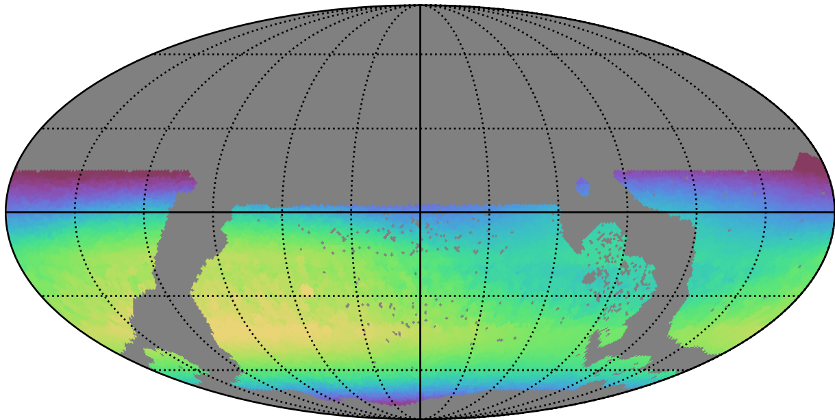
weather_cloudso0v3.4_10yrs WFD i band: Max skyBrightness
