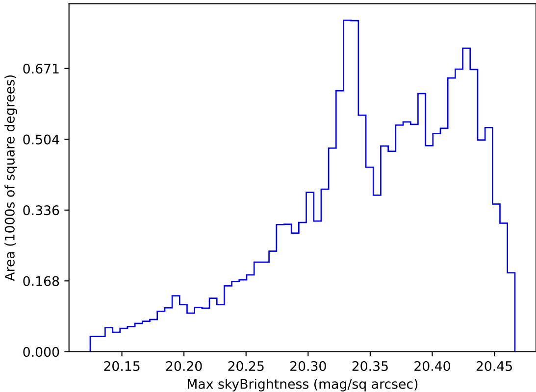
weather_cloudso0v3.4_10yrs WFD i band: Max skyBrightness
