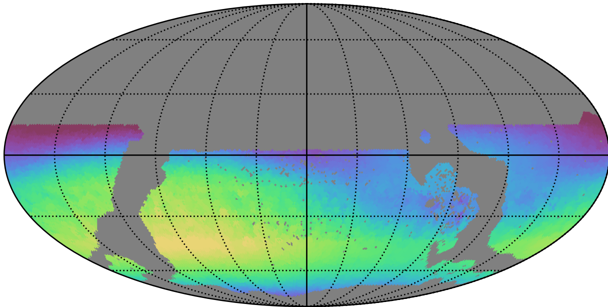
weather_cloudso0v3.4_10yrs WFD all bands: Max skyBrightness
