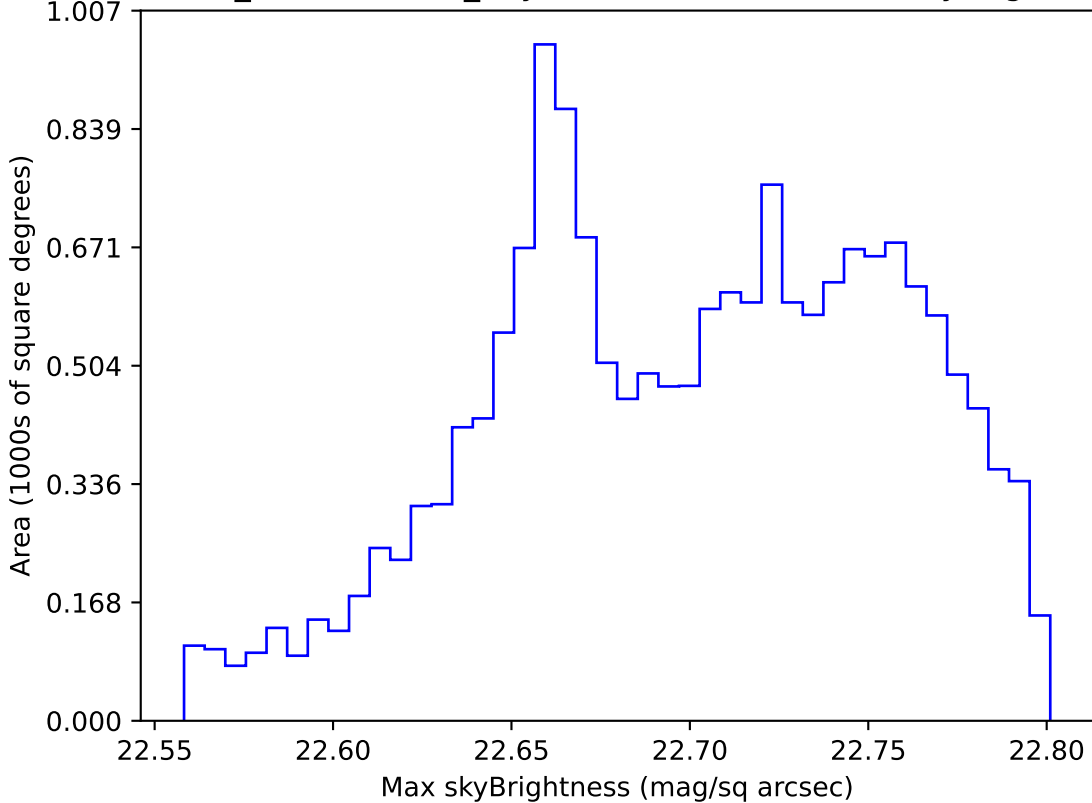
weather_cloudso0v3.4_10yrs WFD all bands: Max skyBrightness
